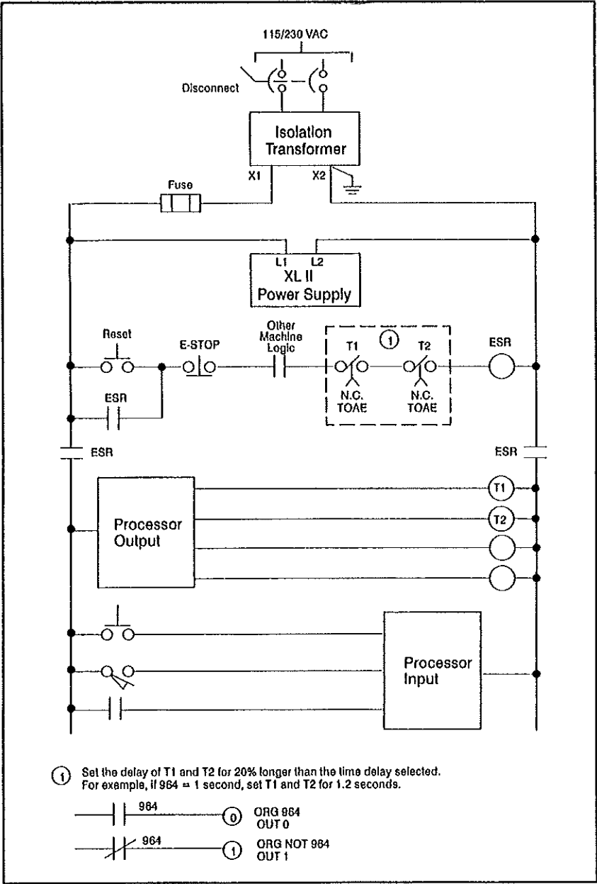
Figure 3.10 - Emergency Stop Wiring
