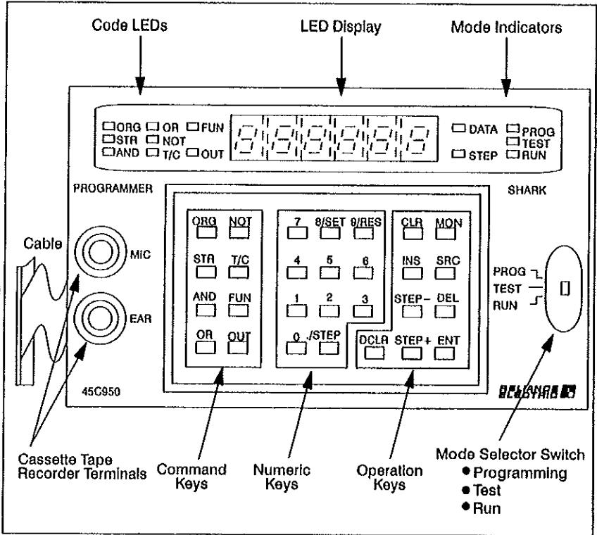
Figure 2.14 - Standard Programmer
