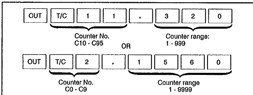
Figure 6.6 - Entering Counter Values
