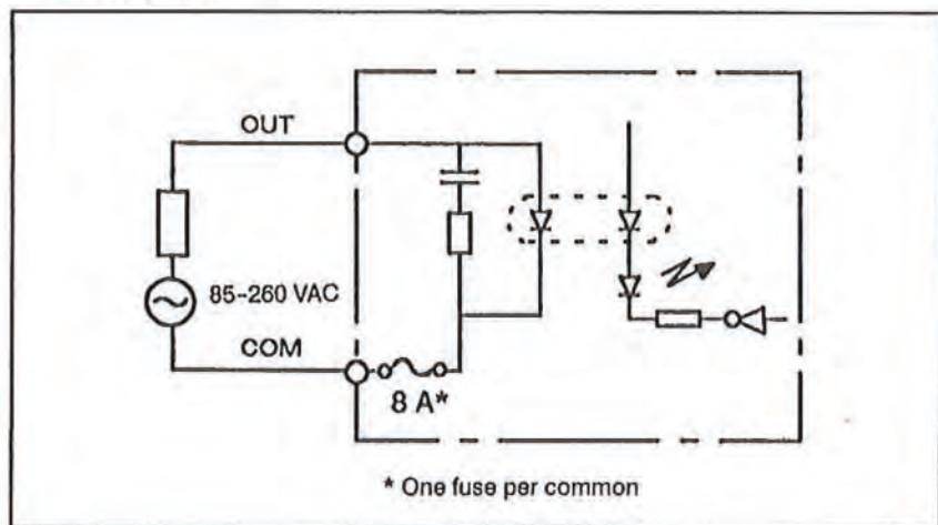
Circuit Diagram
