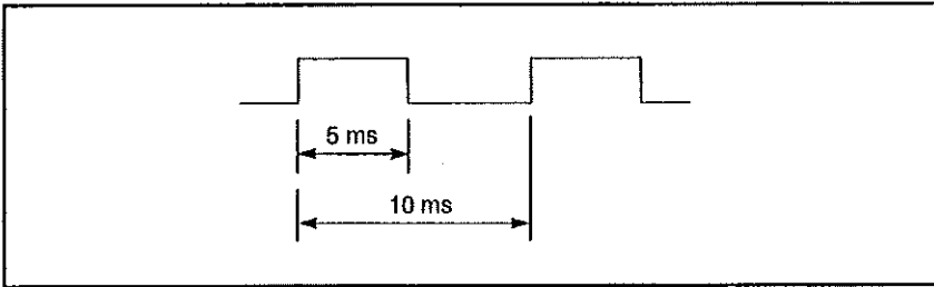
Figure 4.18 - Example of Address 969 Timing
