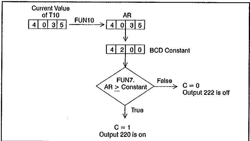
Figure 6.52 - Constant Value Word Comparison ( \geq )
