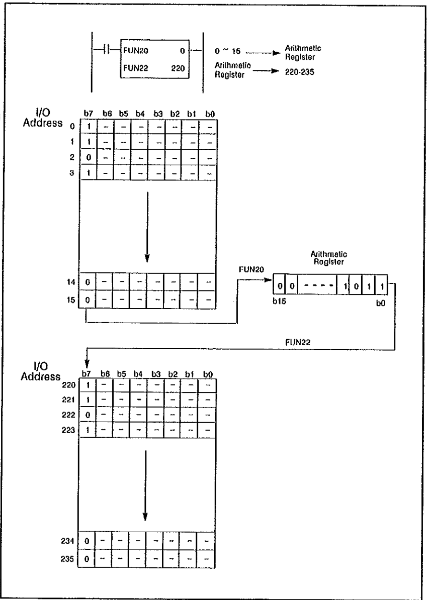
Figure 4.23 - Processing Bits as Words
