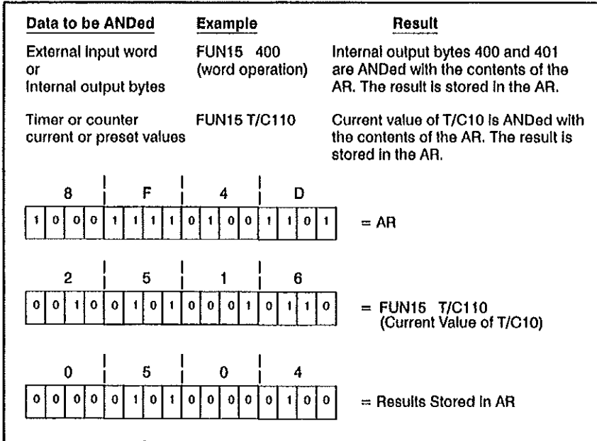
Figure 6.71 - Example of FUN15
