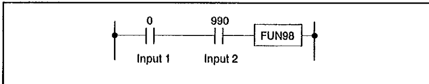
Figure 5.3 - Required Start Sequence
