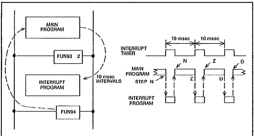
Figure 6.29 - Interrupt Command Operation
