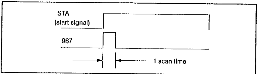
Figure 4.16 - Example of Address 967 Timing
