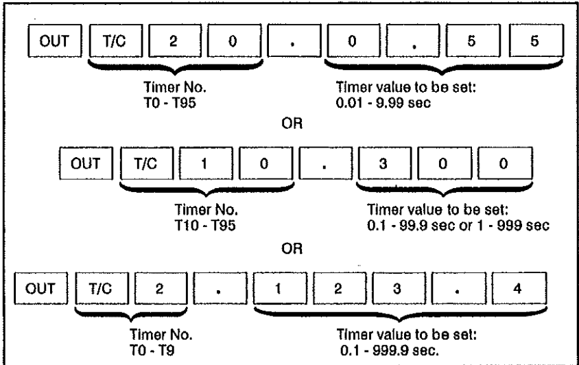
Figure 6.4 - Entering Timer Values
