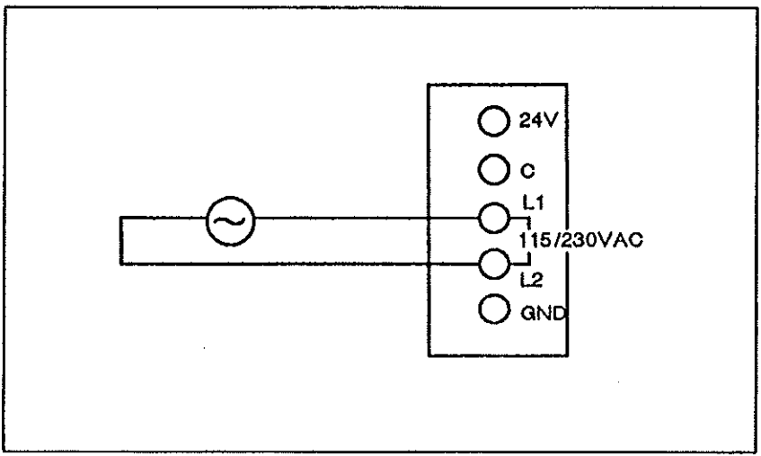
External Wiring
