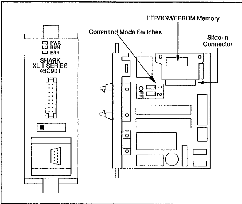
Figure 2.3 - Processor Module
