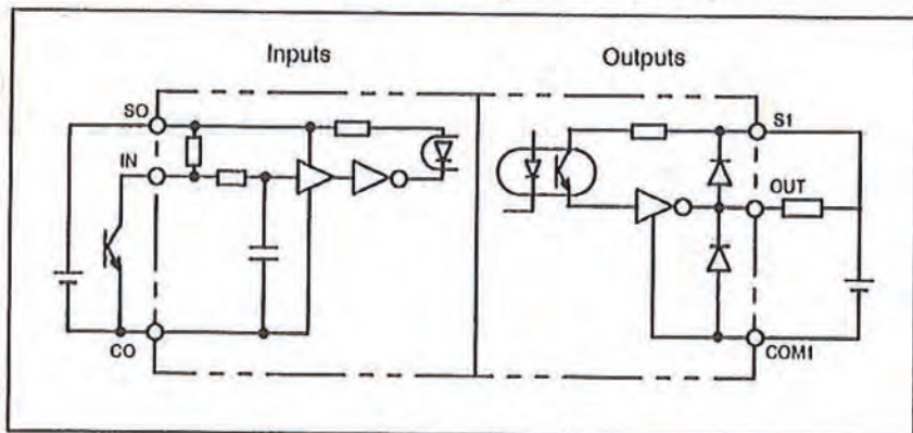
Circuit Diagram
