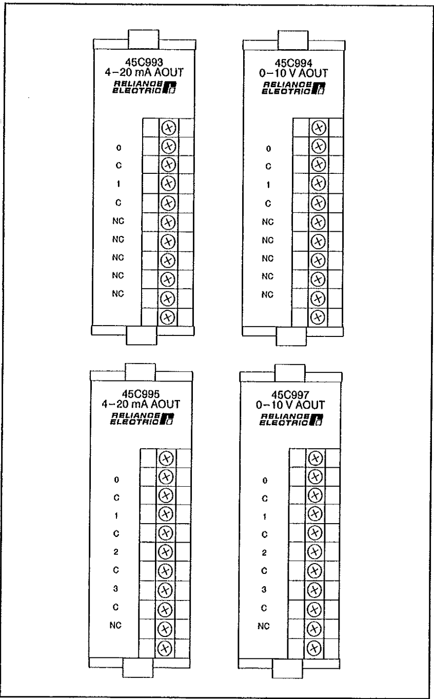
Figure 2.8 - Analog Output Modules
