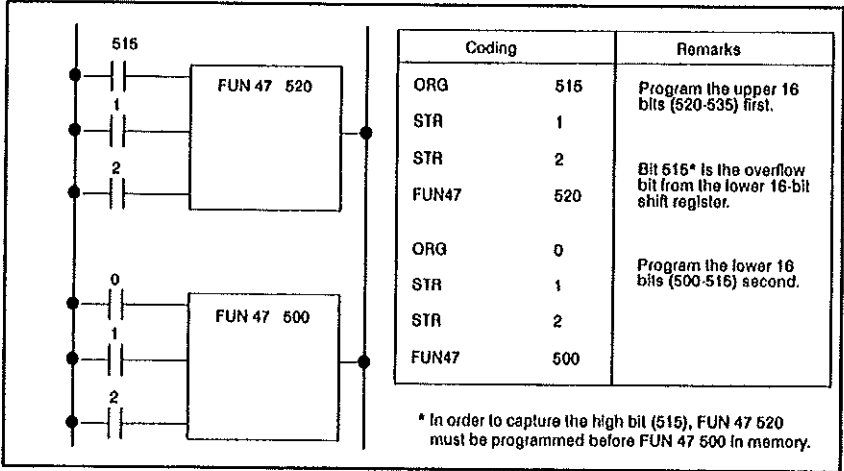
Figure 6.89 - Cascaded Shift Register Example
