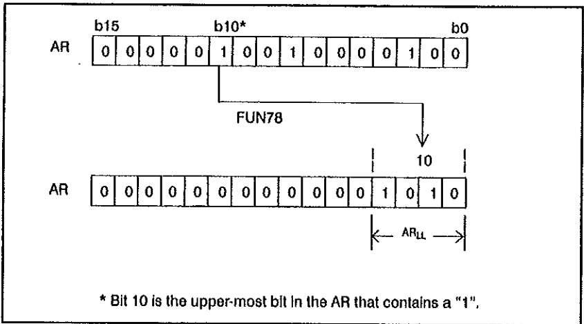
Figure 6.98 - Example of FUN78
