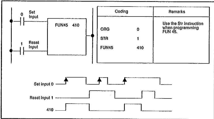
Figure 6.25 - Example of FUN45
