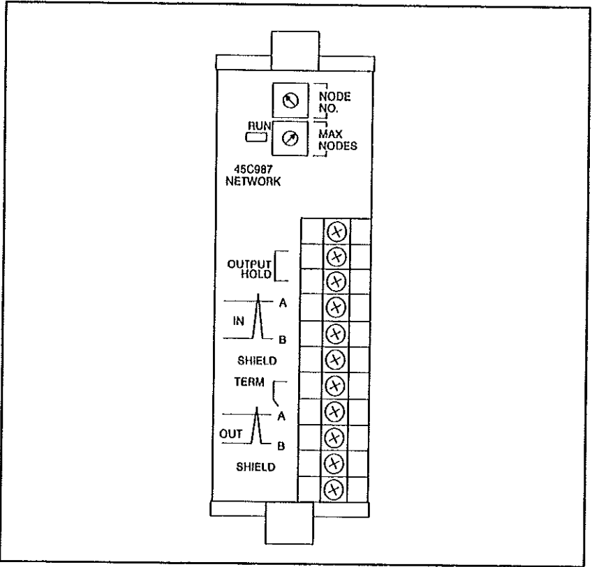
Figure 2.10 - Network Module
