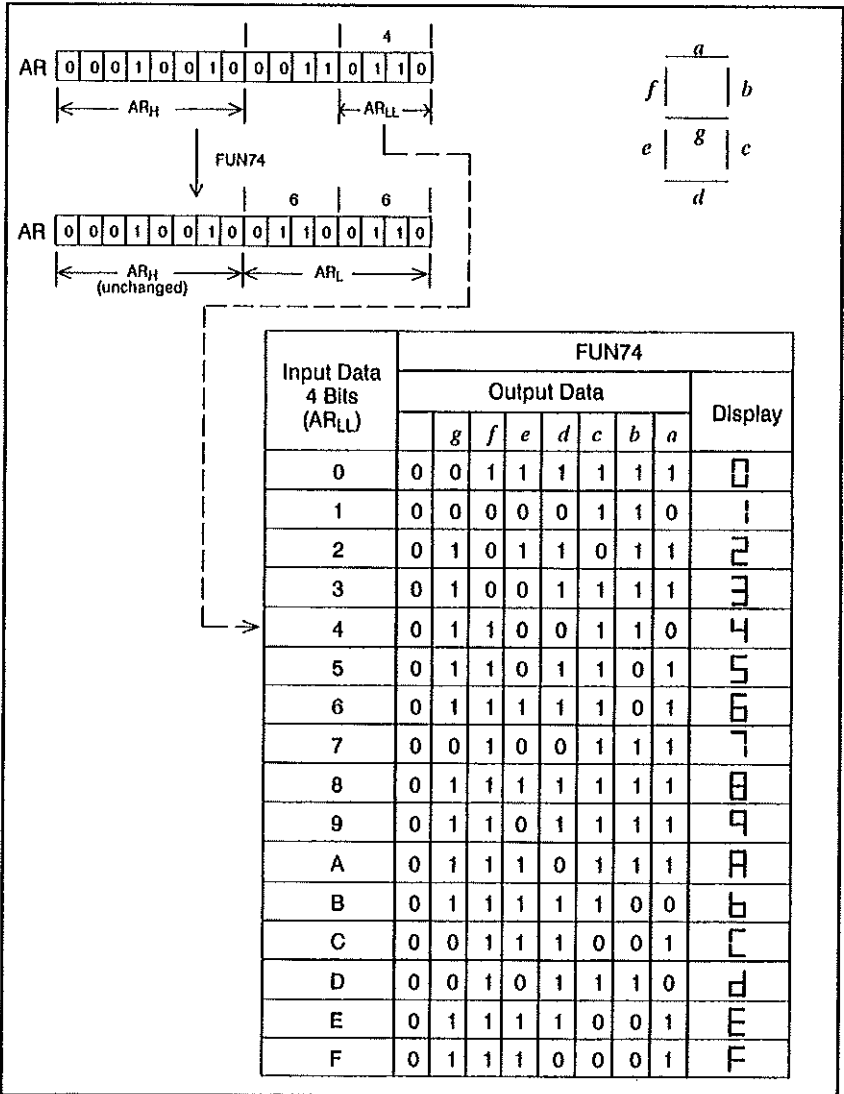
Figure 6.96 - Example of FUN74
