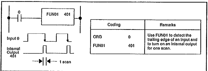
Figure 6.13 - Example of FUN01
