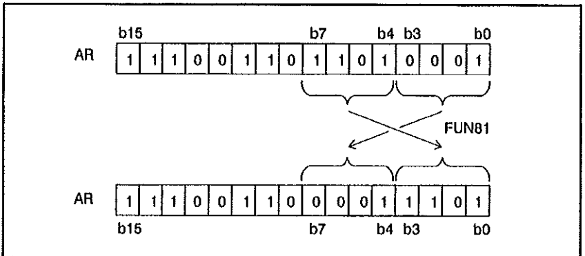
Figure 6.102 - Example of FUN81
