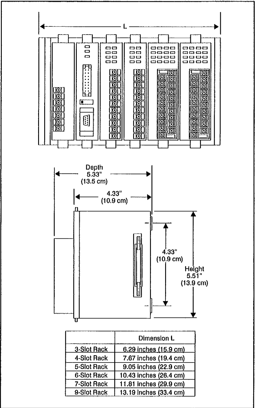
Figure 3.1 - Rack Dimensions
