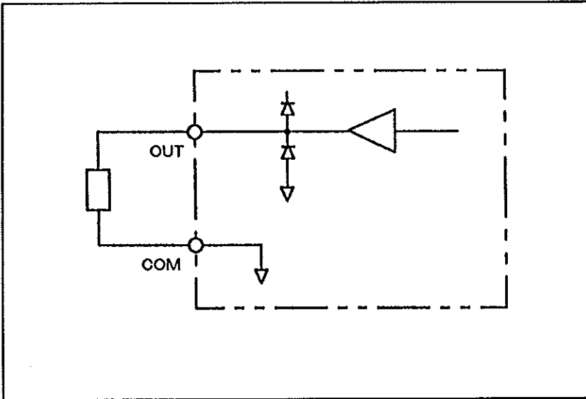
Circuit Diagram
