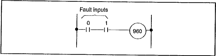
Figure 4.9 – Example of Address 960 Programming
