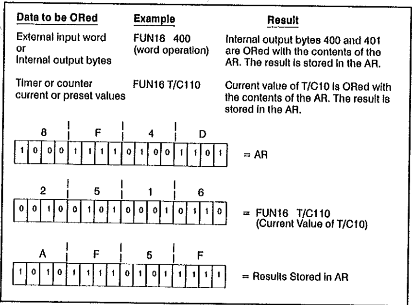
Figure 6.73 - Example of FUN16
