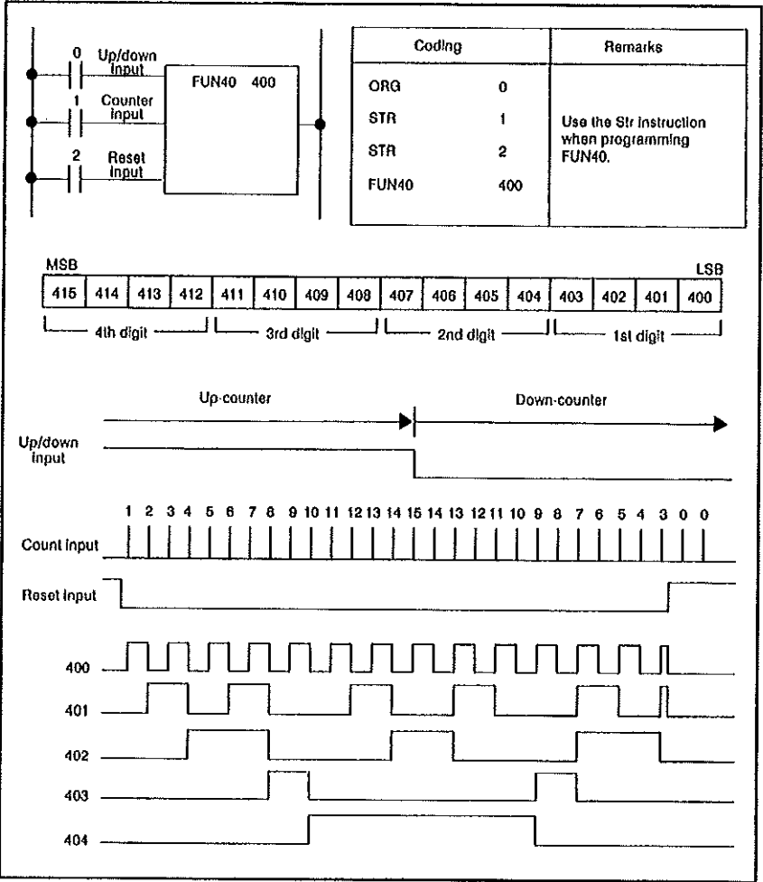
Figure 8.94 - Example of FUN40
