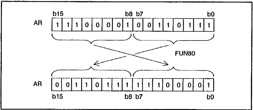
Figure 6.101 - Example of FUN80
