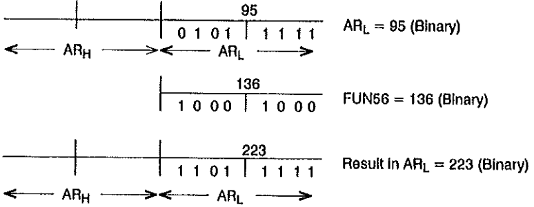
Figure 6.49 - Example of FUN56
