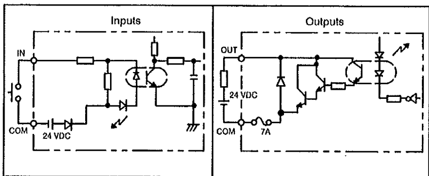
Circuit Diagram
