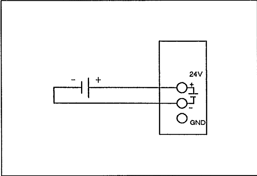
External Wiring
