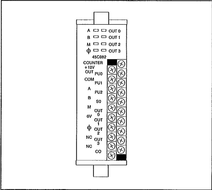
Figure 2.9 - Counter Module
