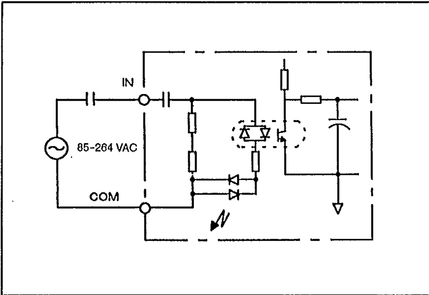
Circuit Diagram
