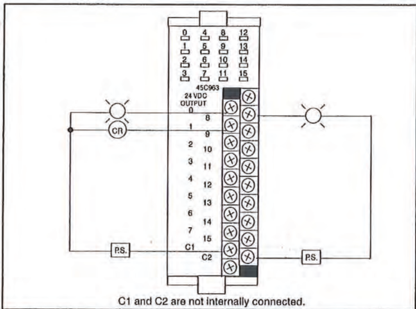
Figure 3.15 - 24 VDC Output Module Wiring (M/N 45C962, 45C963, and 45C964)
