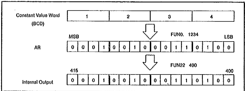
Figure 6.34 - Constant Value Word Load
