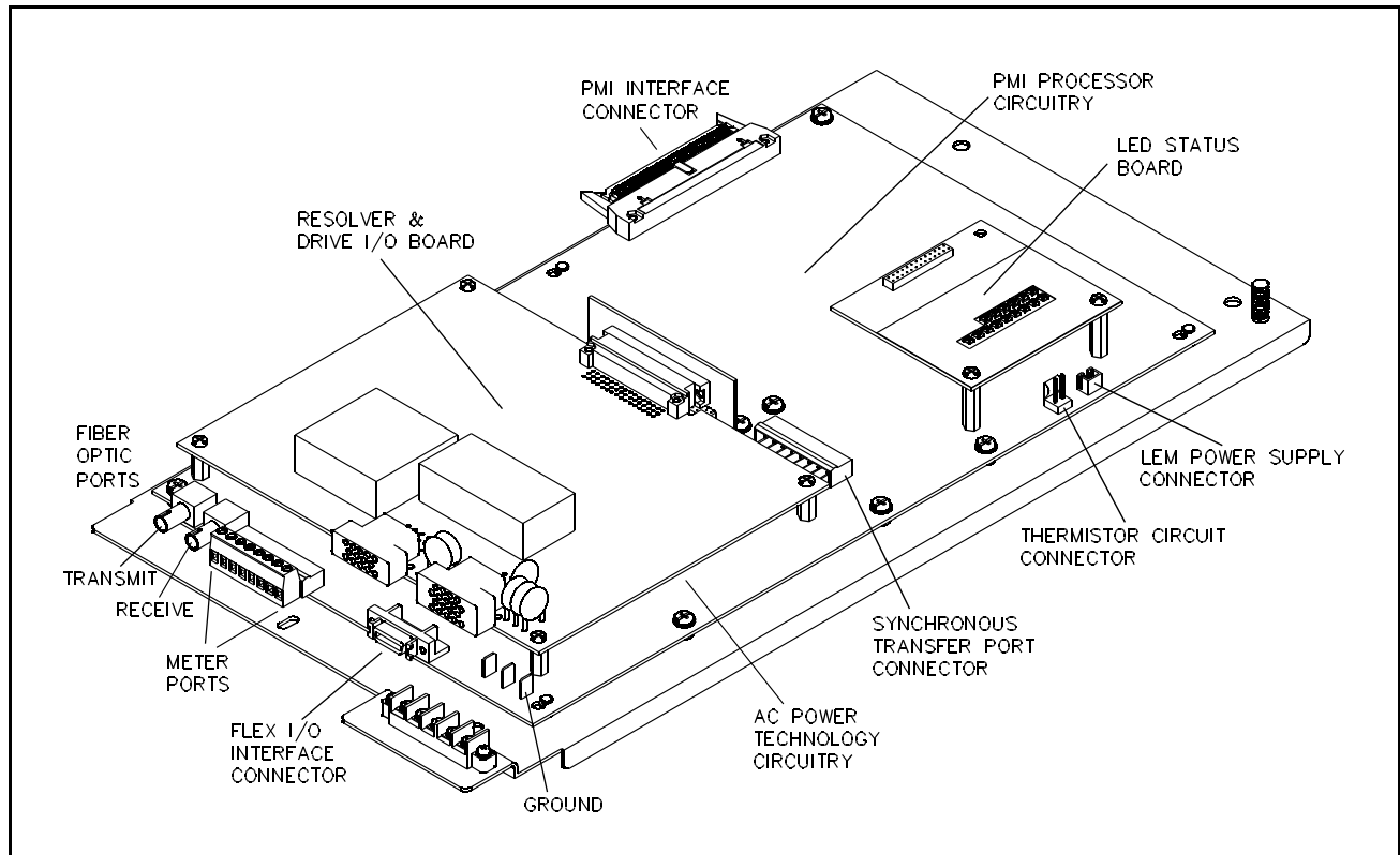
Figure 2.7 – SA3100 PMI Regulator
