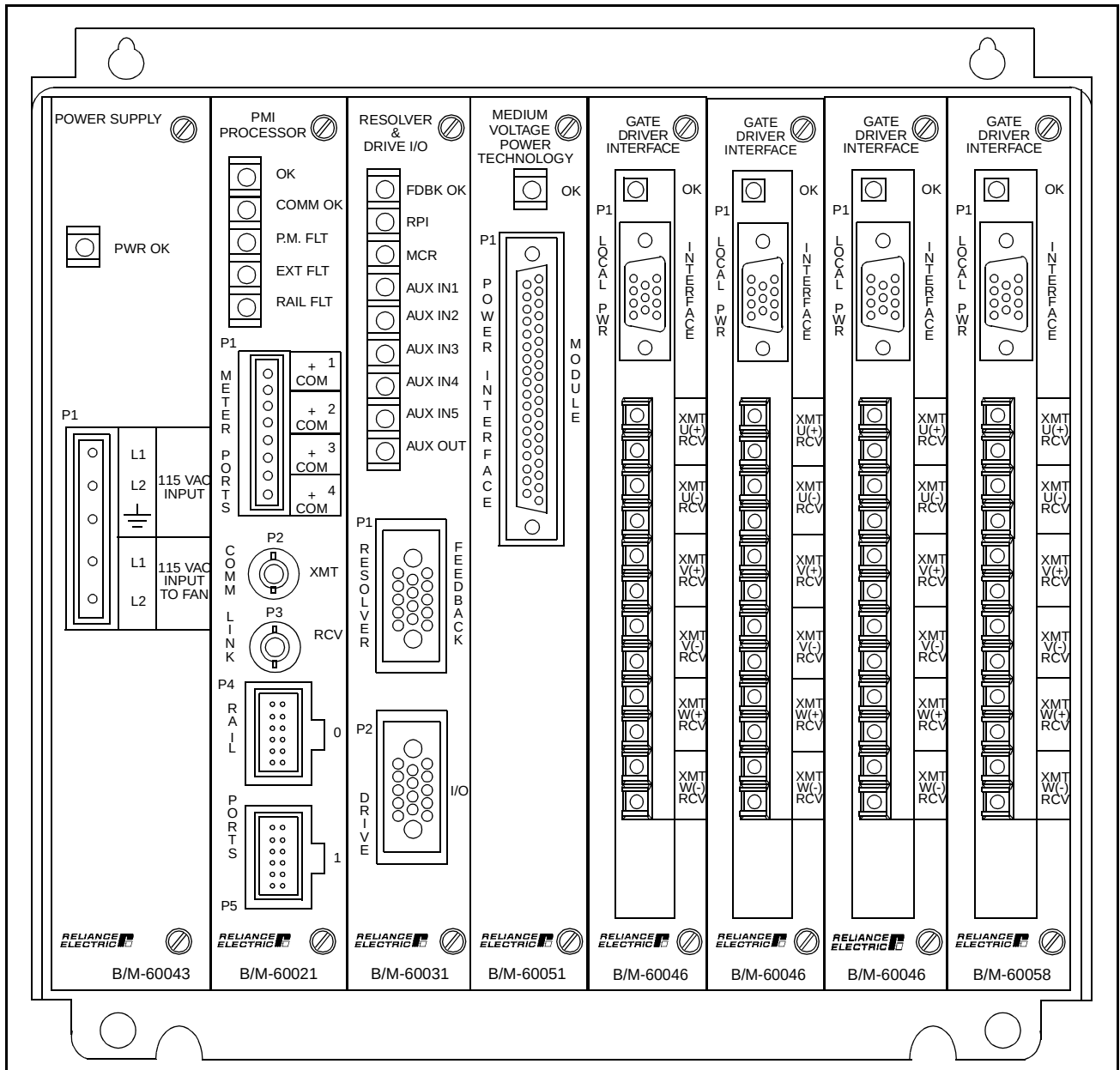
Figure 2.8 – Eight-Slot PMI Rack and Modules (1567 Power Max™ Drives)
