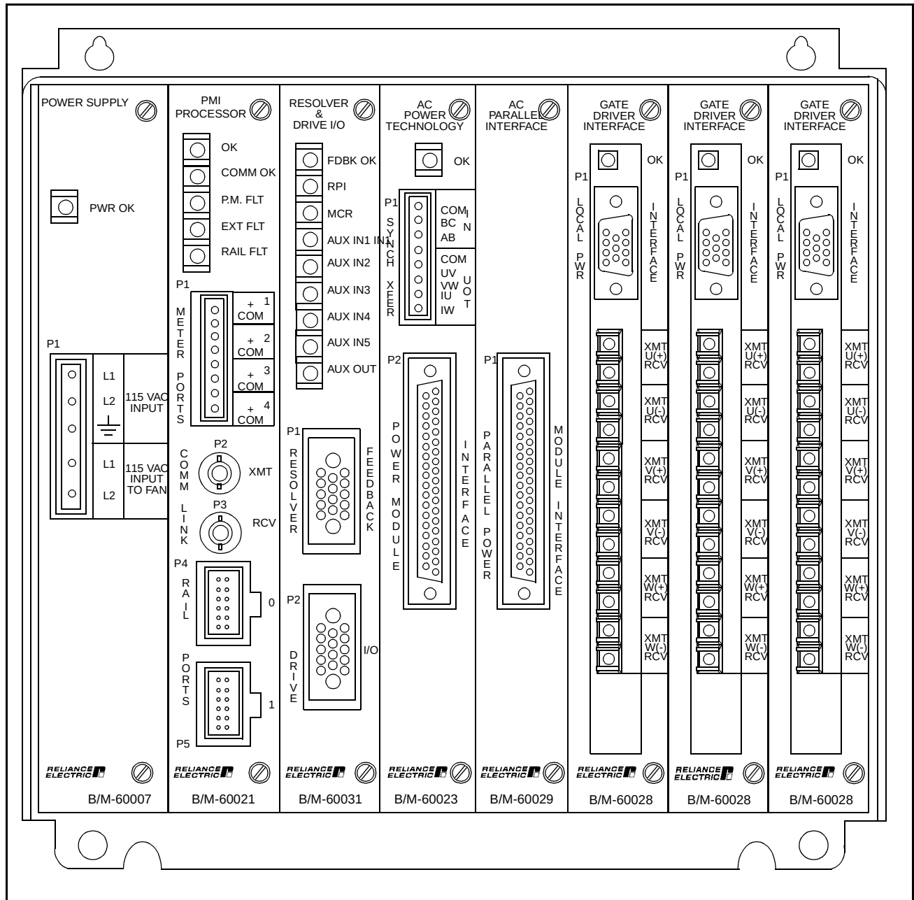
Figure 2.6 – Eight-Slot PMI Rack and Modules (SA3000 High Power Drives)
