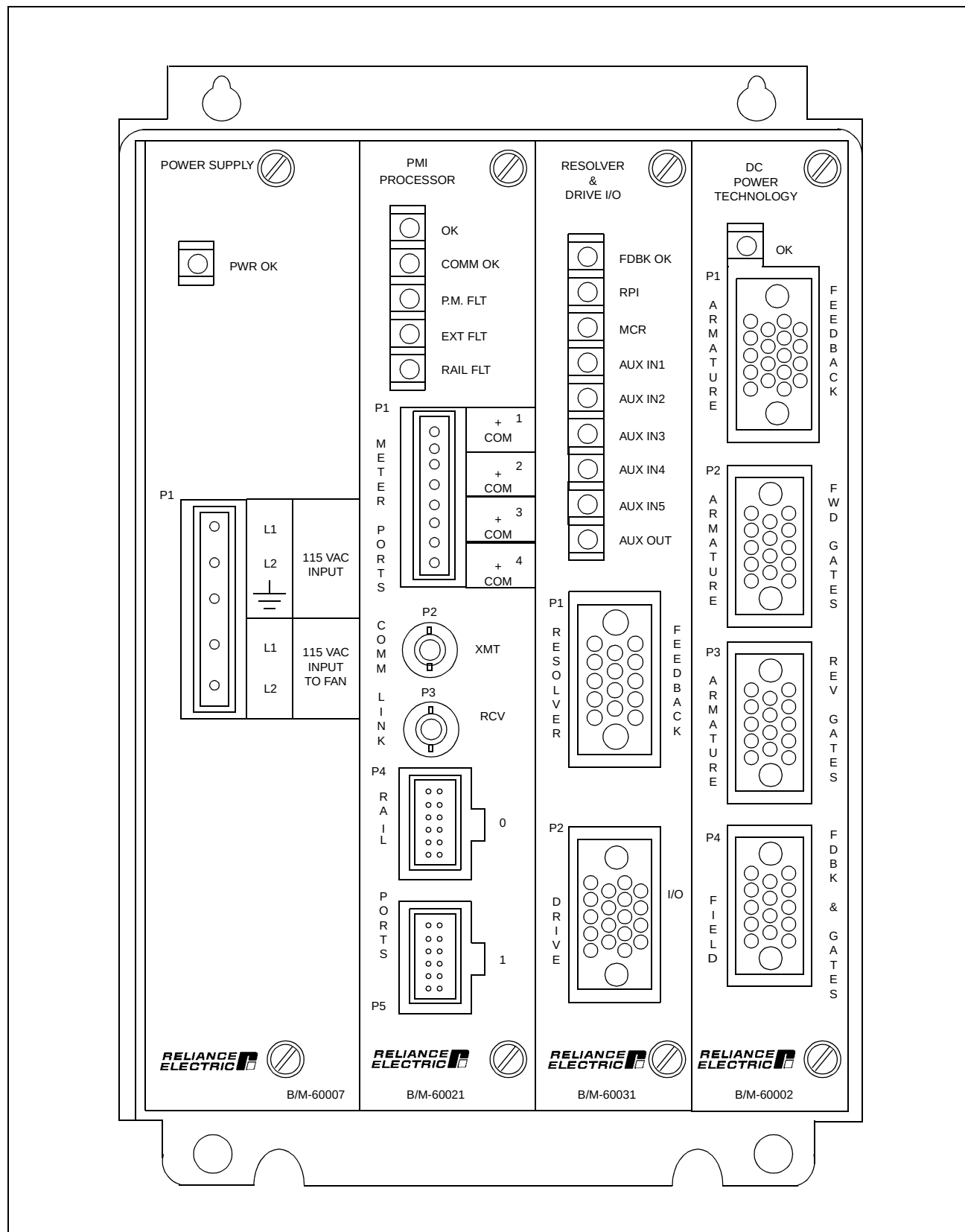
Figure 2.3 – Four-Slot PMI Rack and Modules (SD300/SF3000 Drives)
