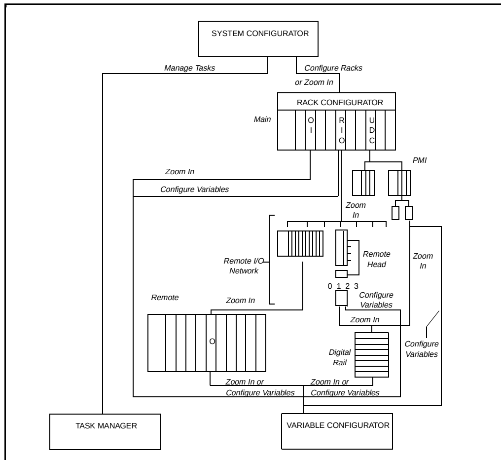
Figure 3.1 – AutoMax Executive Off-Line Programming Applications
