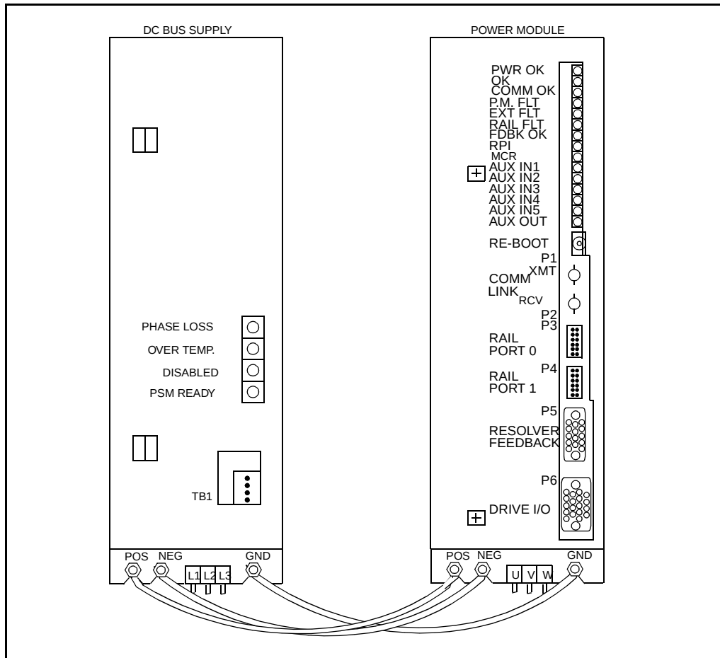
Figure 2.4 – SA500 DC Bus Supply and Power Module
