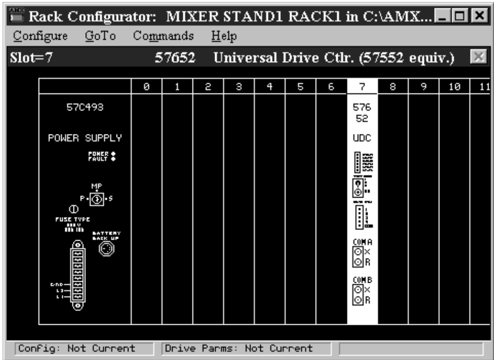
Figure 3.2 – Adding a Module
