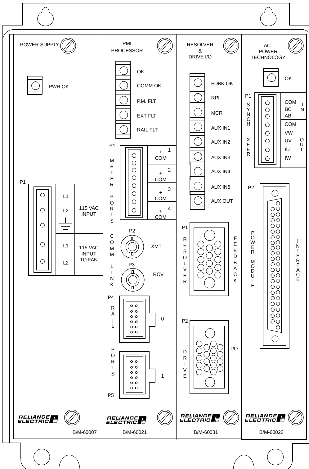
Figure 2.5 – Four-Slot PMI Rack and Modules (SA3000 Medium Power Drives)
